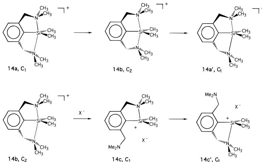
Figure 4. HF/6-31G(d) (normal print), B3LYP/6-31G(d) (underlined italics), and SCIPCM-B3LYP/6-31G(d) ( \epsilon(\text{CH}_3\text{OH}) = 32.6 ; underlined italics in parentheses) geometrical parameters of (a) 14a , (b) 14b , and (c) 14c . Bond lengths are in Å, angles in deg.
