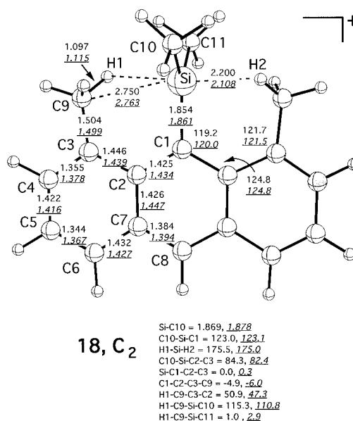
Figure 8. HF/6-31G(d) (normal print) and B3LYP/6-31G(d) (underlined italics) geometrical parameters of cation 18 . Bond lengths are in Å, angles in deg.
