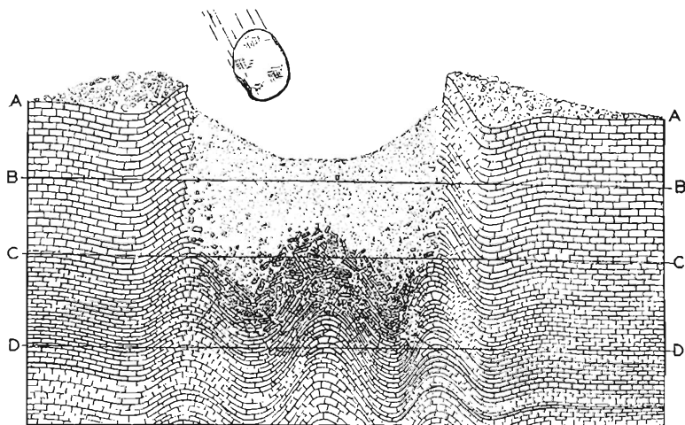
Fig. 2. Ideal section through a meteorite crater according to the writers' concept of structures produced by impact and explosion. (For explanation of lettered lines see text.) Relative size of a meteorite believed to be capable of forming the scar shown is indicated above the crater.
